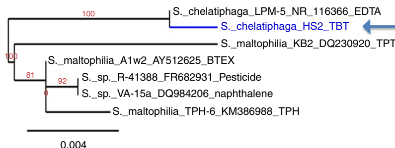
Figure 3 Phylogenetic tree based on 16S rRNA gene sequences showing the relationship with Stenotrophomonas chelatiphaga HS2 strain (accession number KR780649) pointed by an arrow to other reported Stenotrophomonas strains. The strain followed by the accession numbers and degraded substrate; petroleum hydrocarbon (petroleum H), benzene (BTEX), toluene, ethylbenzene and xylenes, triphenyltin (TPT), ethylenediaminetetra acetic acid (EDTA), and tributyltin (TBT) degraders.
